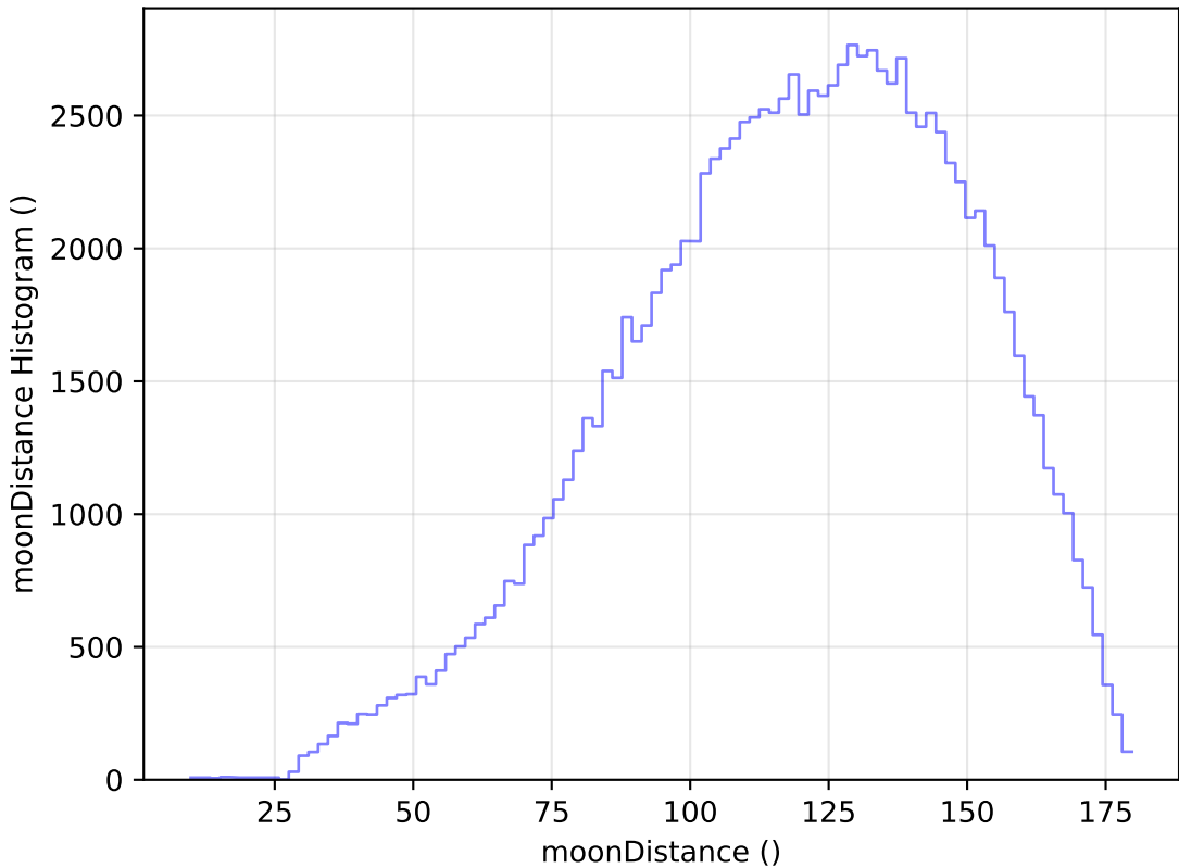
roll_pause_mjdp120_v3.4_10yrs All sky u band: moonDistance Histogram
