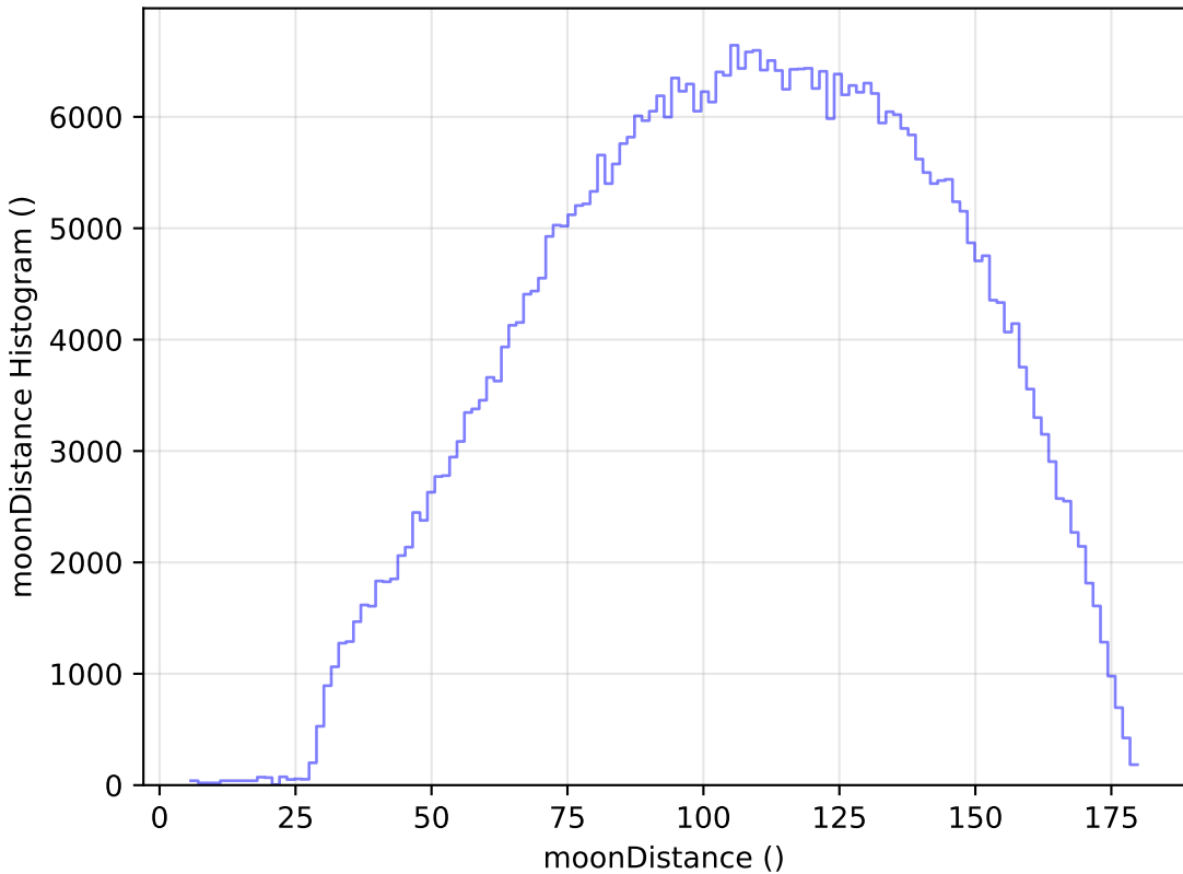
roll_pause_mjdp120_v3.4_10yrs All sky r band: moonDistance Histogram
