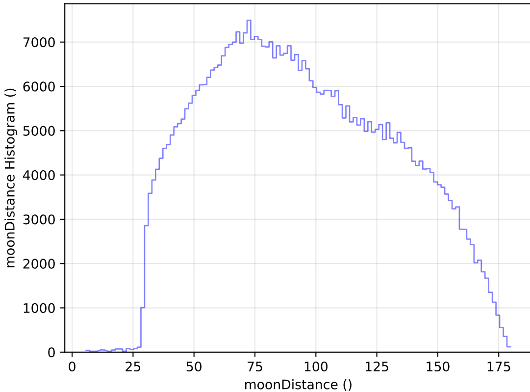
roll_pause_mjdp120_v3.4_10yrs All sky i band: moonDistance Histogram
