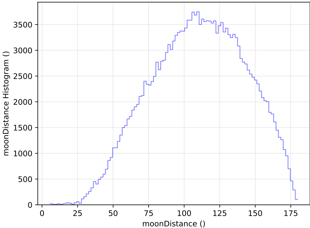
roll_pause_mjdp120_v3.4_10yrs All sky g band: moonDistance Histogram
