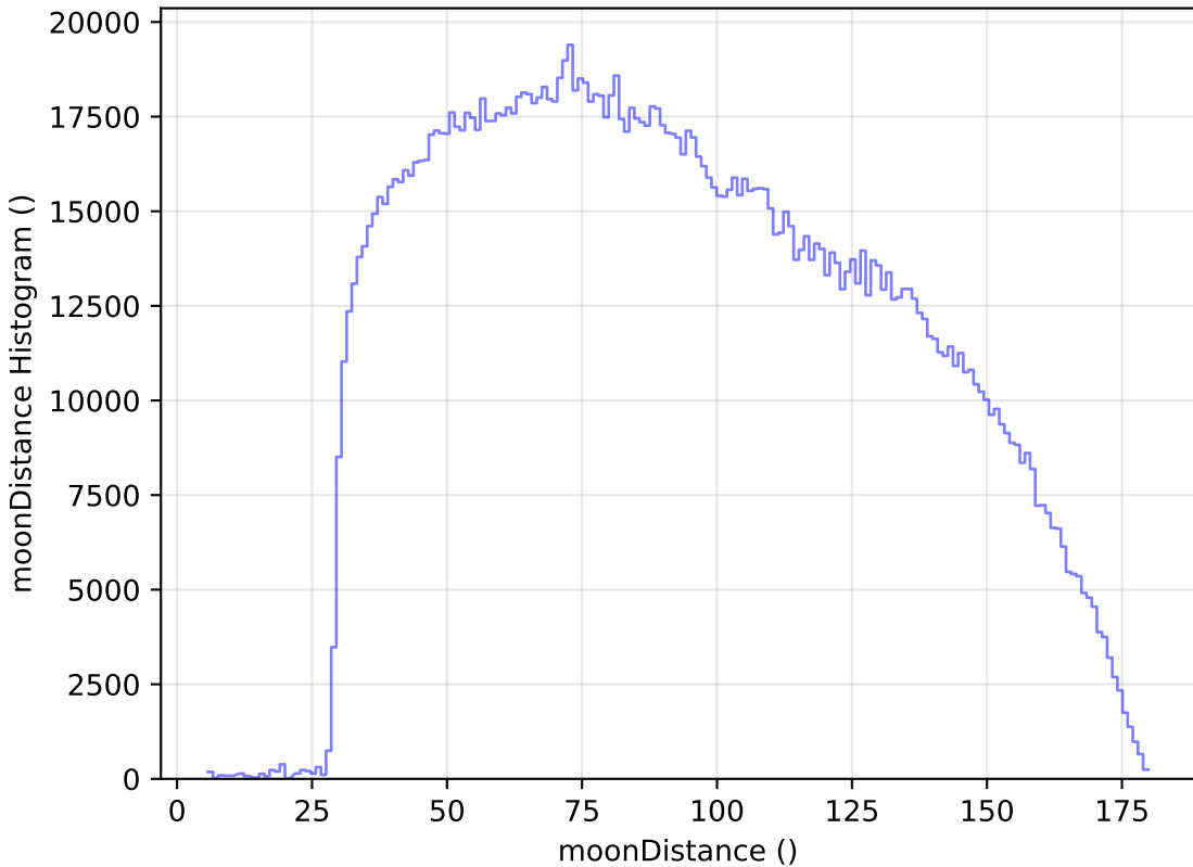
roll_pause_mjdp120_v3.4_10yrs All sky all bands: moonDistance Histogram
