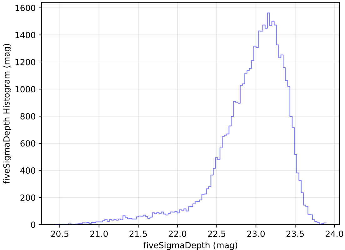
roll_pause_mjdp120_v3.4_10yrs Yr 1 z band: fiveSigmaDepth Histogram
