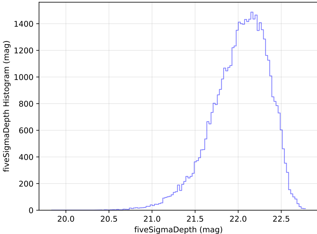
roll_pause_mjdp120_v3.4_10yrs Yr 1 y band: fiveSigmaDepth Histogram
