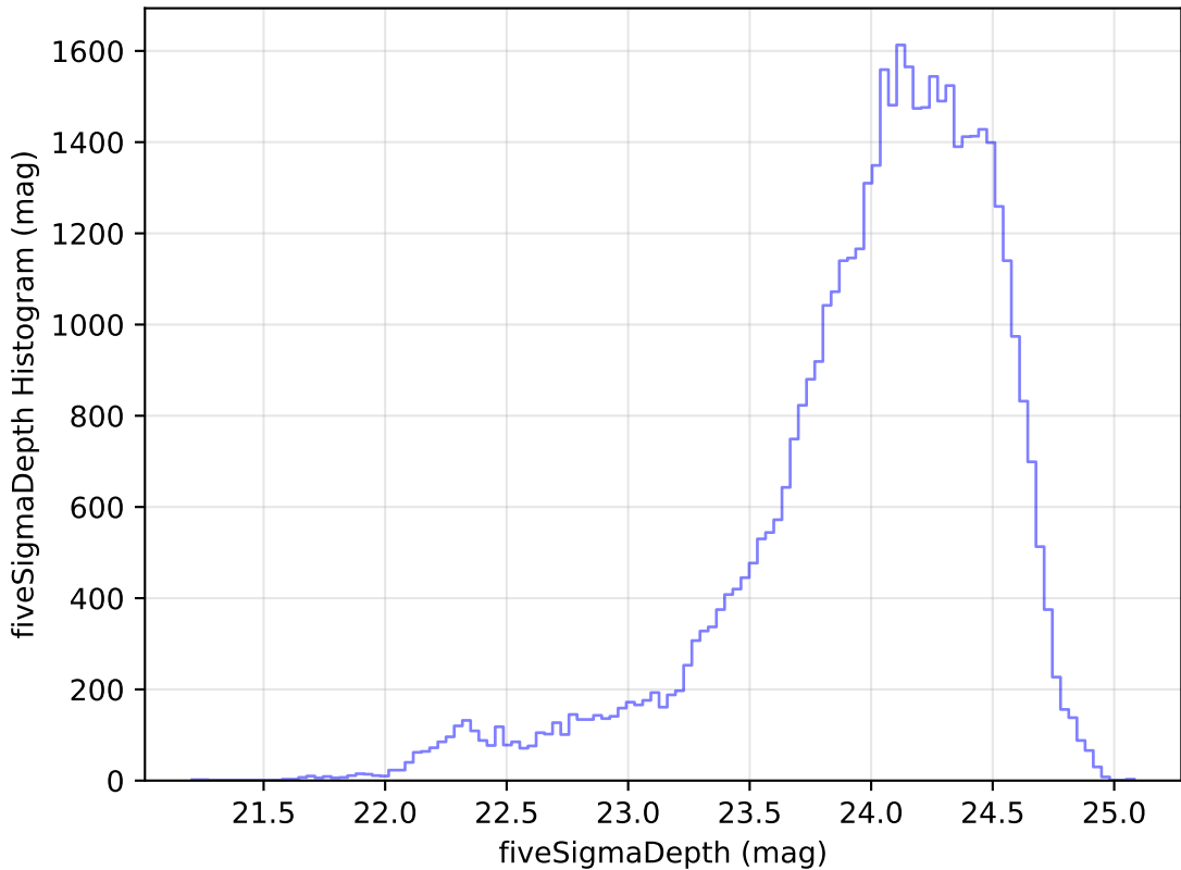
roll_pause_mjdp120_v3.4_10yrs Yr 1 r band: fiveSigmaDepth Histogram
