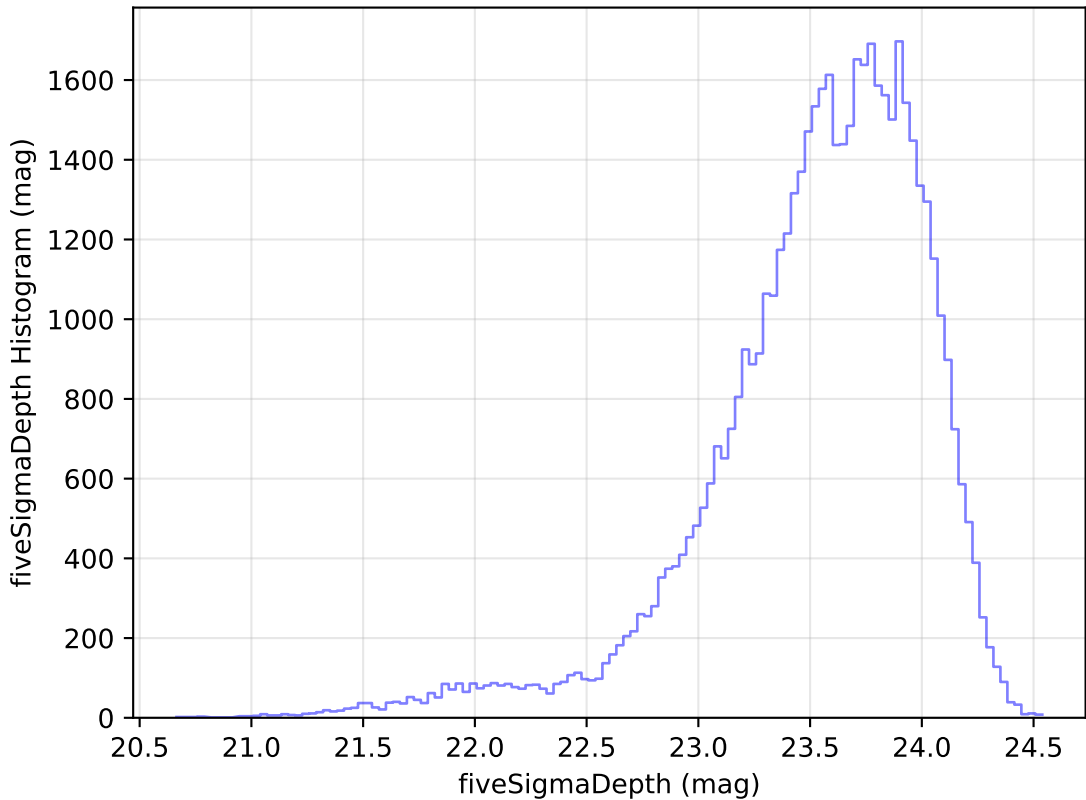
roll_pause_mjdp120_v3.4_10yrs Yr 1 i band: fiveSigmaDepth Histogram
