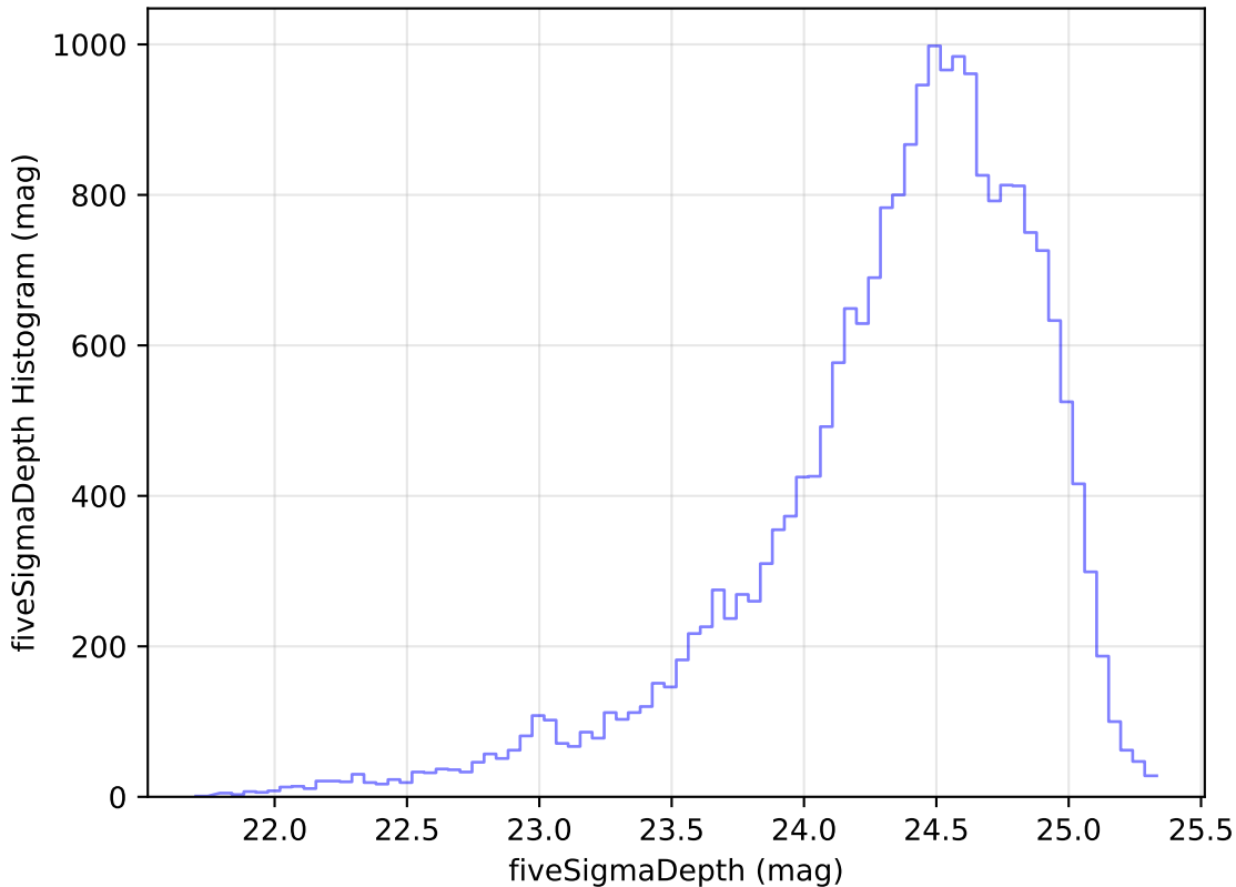
roll_pause_mjdp120_v3.4_10yrs Yr 1 g band: fiveSigmaDepth Histogram
