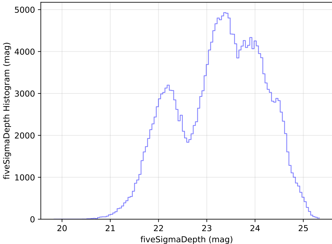
roll_pause_mjdp120_v3.4_10yrs Yr 1 all bands: fiveSigmaDepth Histogram
