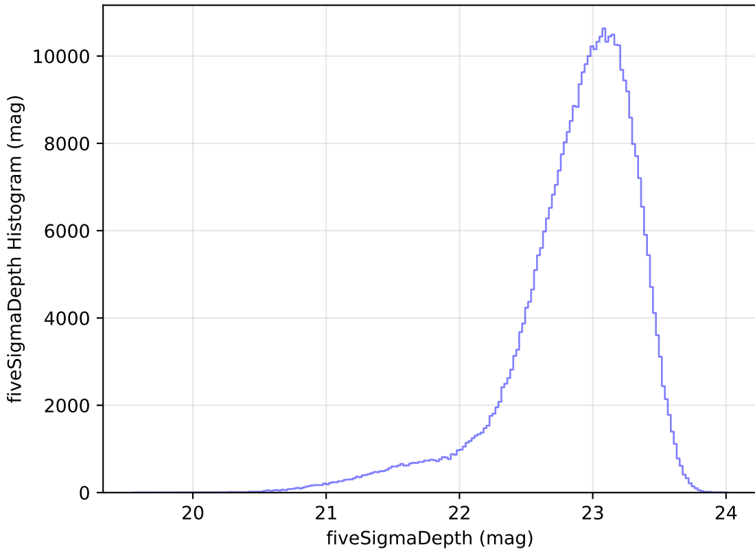
roll_pause_mjdp120_v3.4_10yrs WFD z band: fiveSigmaDepth Histogram
