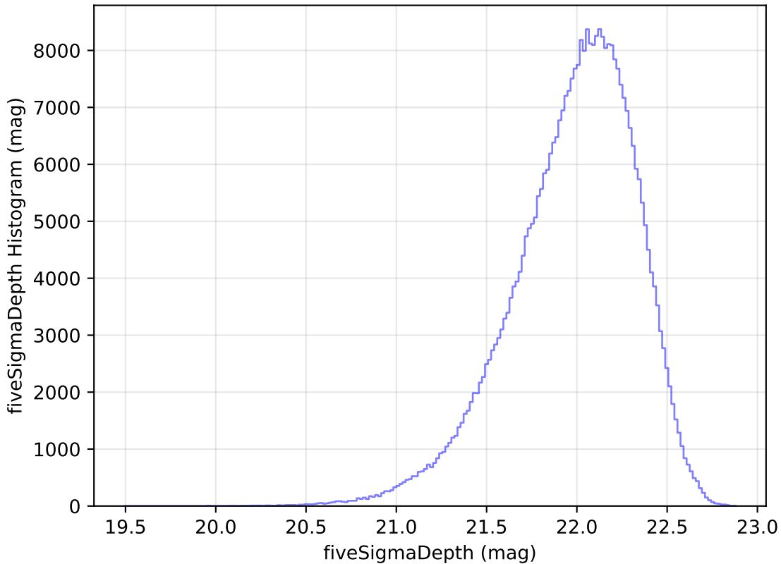
roll_pause_mjdp120_v3.4_10yrs WFD y band: fiveSigmaDepth Histogram
