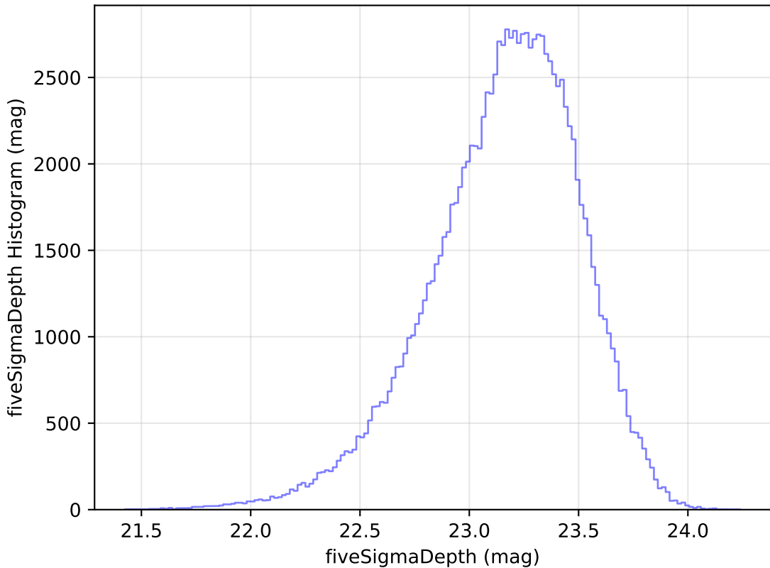
roll_pause_mjdp120_v3.4_10yrs WFD u band: fiveSigmaDepth Histogram
