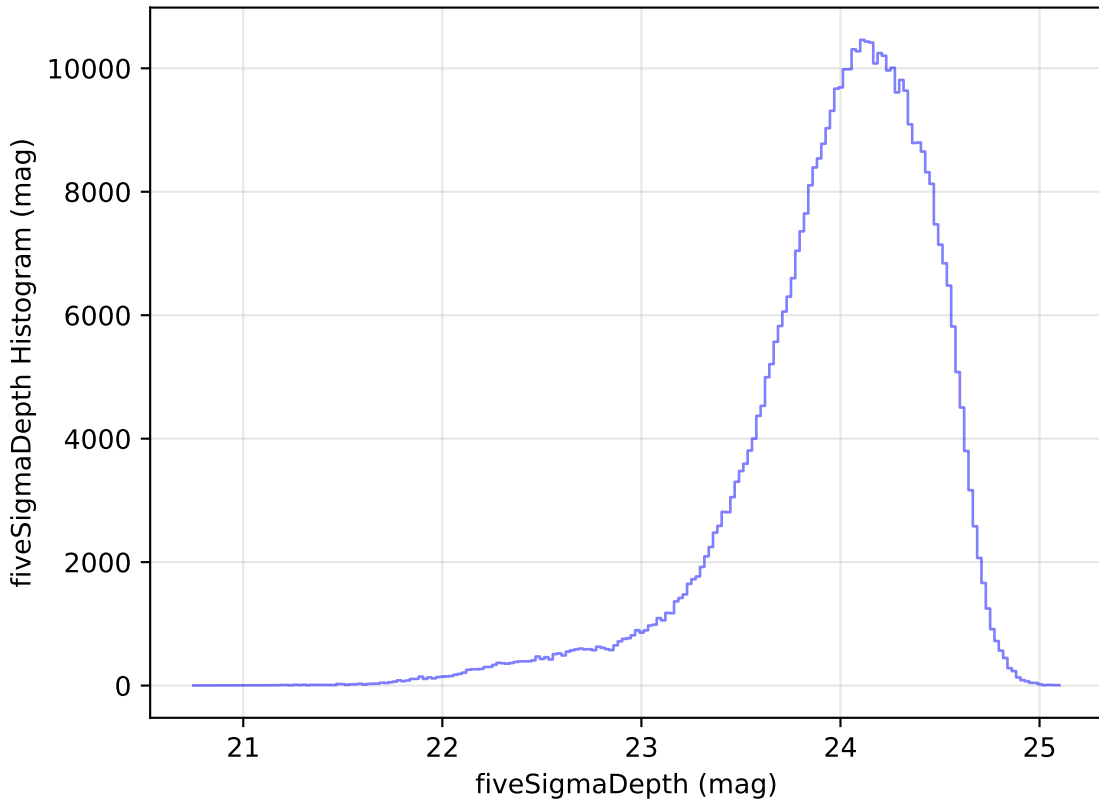
roll_pause_mjdp120_v3.4_10yrs WFD r band: fiveSigmaDepth Histogram
