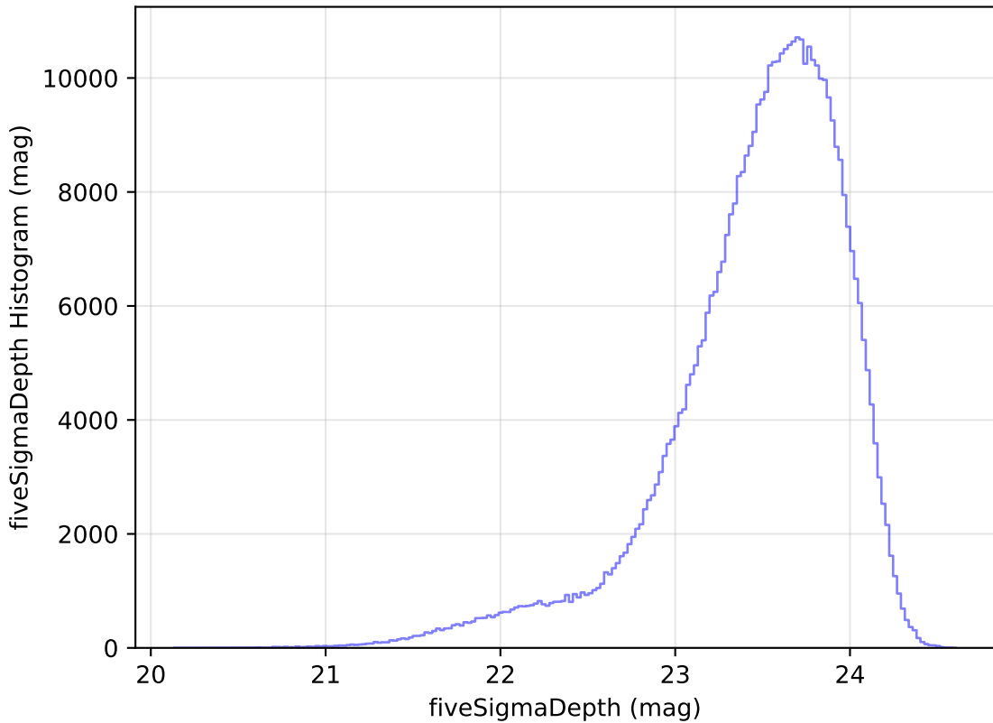
roll_pause_mjdp120_v3.4_10yrs WFD i band: fiveSigmaDepth Histogram
