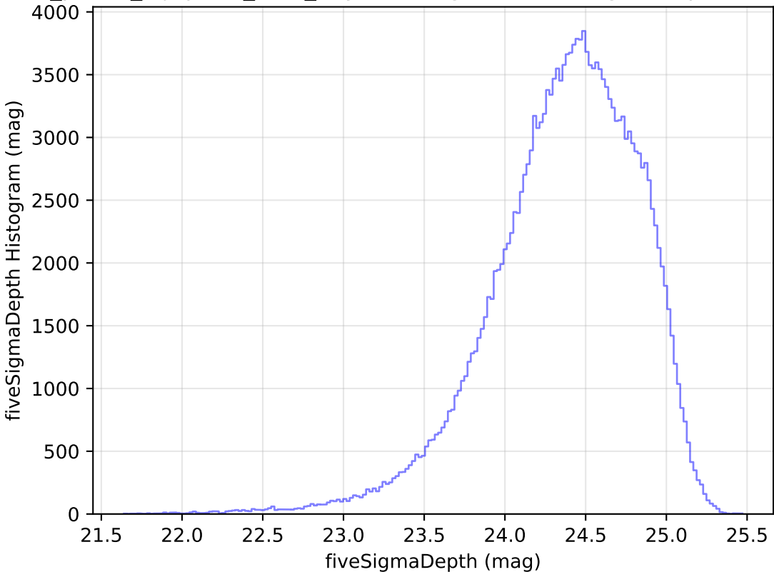
roll_pause_mjdp120_v3.4_10yrs WFD g band: fiveSigmaDepth Histogram
