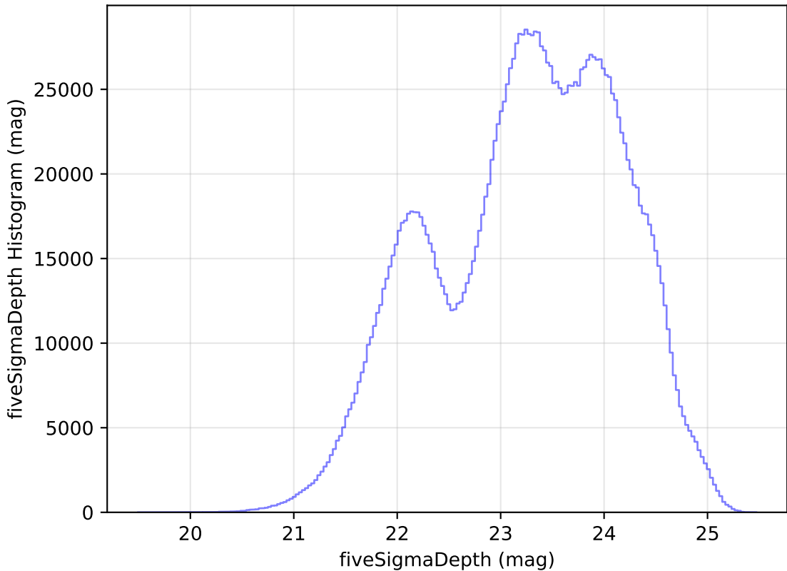
roll_pause_mjdp120_v3.4_10yrs WFD all bands: fiveSigmaDepth Histogram
