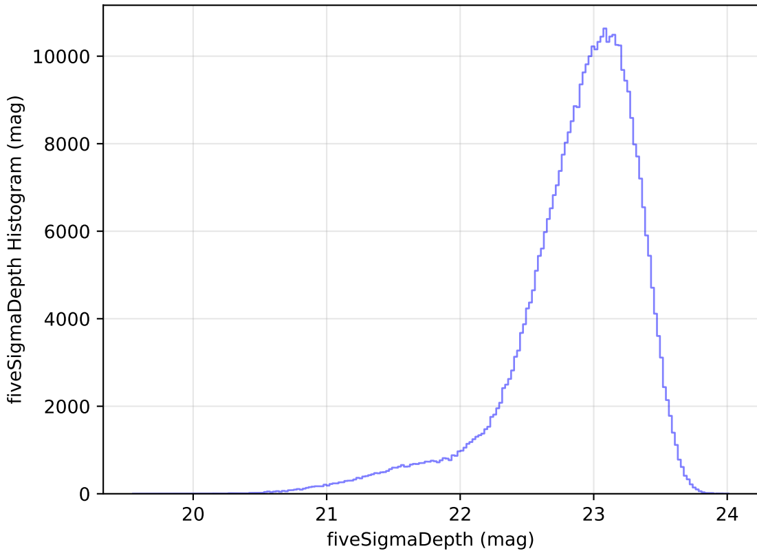
roll_pause_mjdp120_v3.4_10yrs All sky z band: fiveSigmaDepth Histogram
