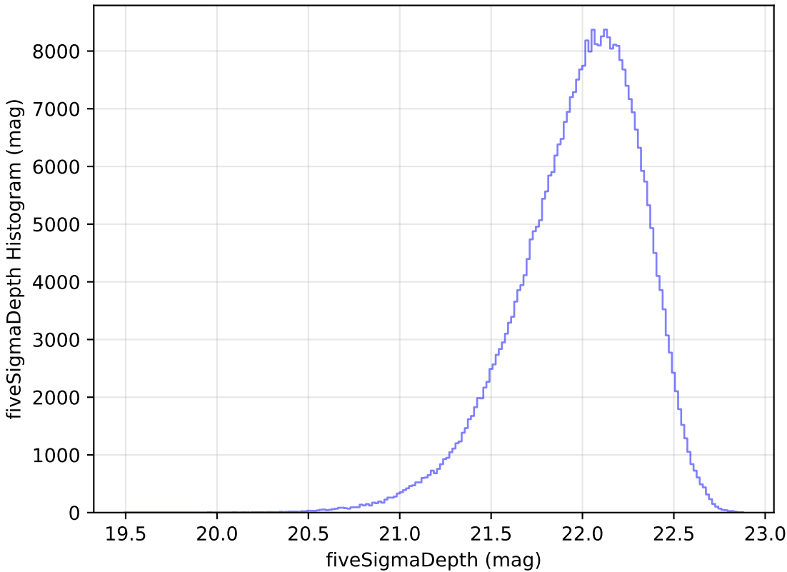
roll_pause_mjdp120_v3.4_10yrs All sky y band: fiveSigmaDepth Histogram
