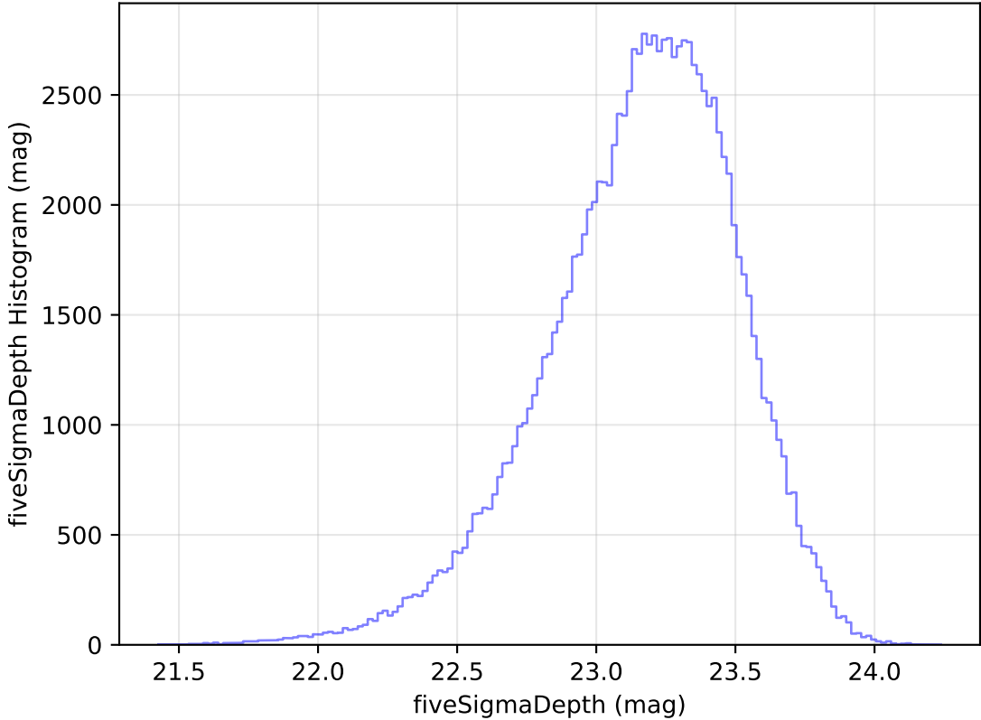
roll_pause_mjdp120_v3.4_10yrs All sky u band: fiveSigmaDepth Histogram
