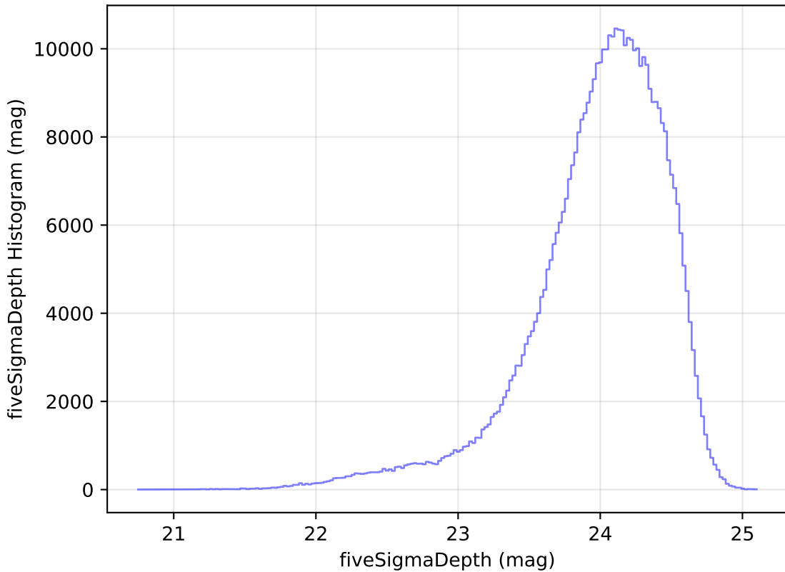
roll_pause_mjdp120_v3.4_10yrs All sky r band: fiveSigmaDepth Histogram
