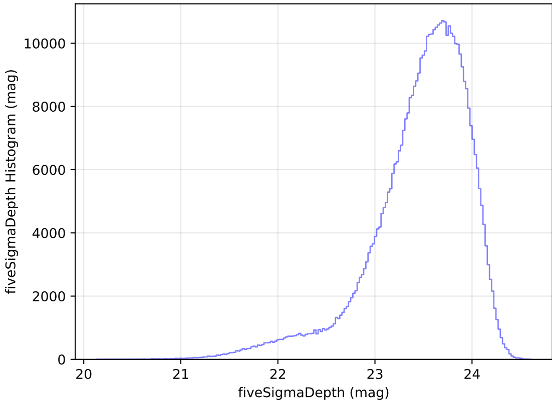
roll_pause_mjdp120_v3.4_10yrs All sky i band: fiveSigmaDepth Histogram
