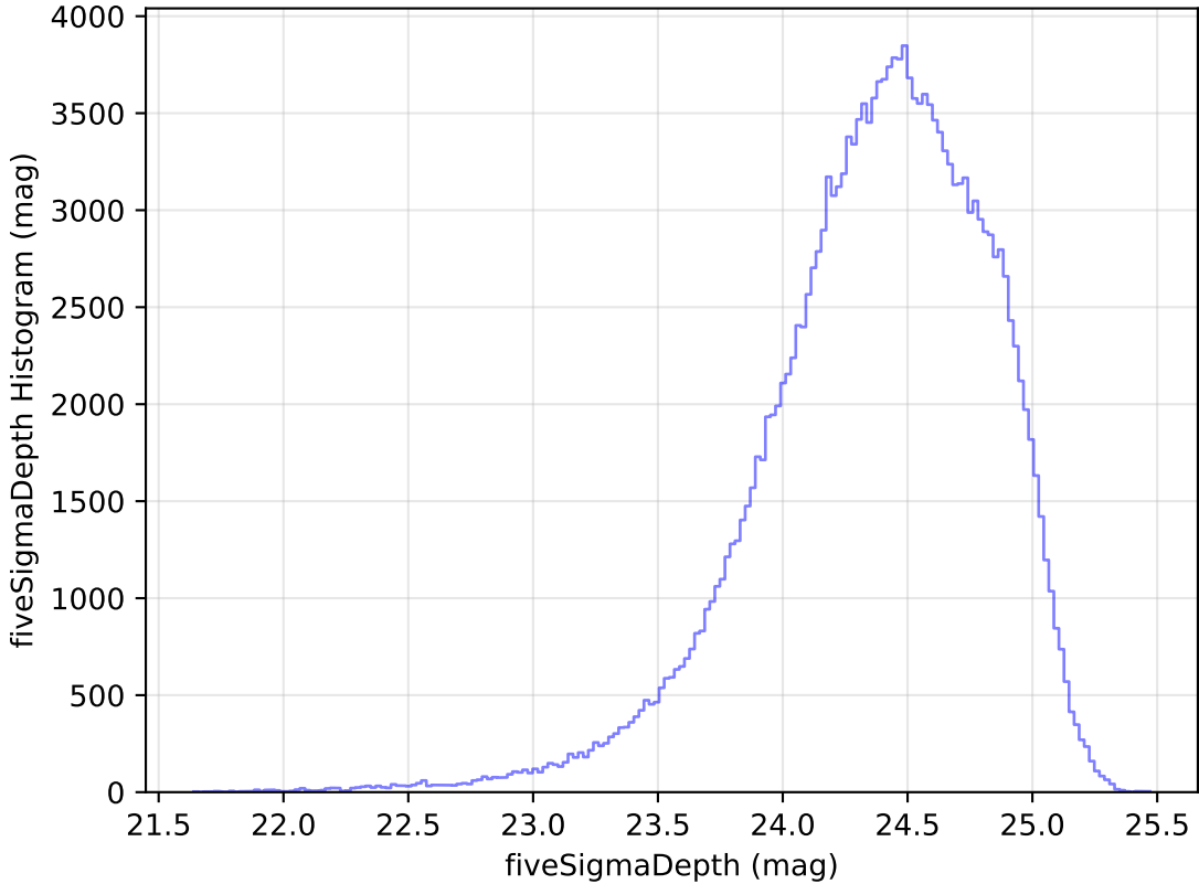
roll_pause_mjdp120_v3.4_10yrs All sky g band: fiveSigmaDepth Histogram
