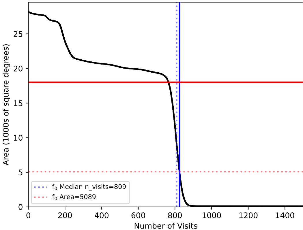
roll_pause_mjdp120_v3.4_10yrs All sky: fO
