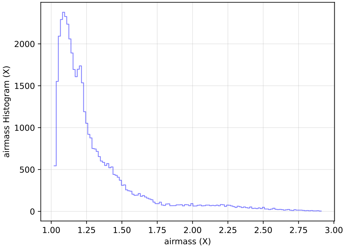
roll_pause_mjdp120_v3.4_10yrs Yr 1 z band: airmass Histogram
