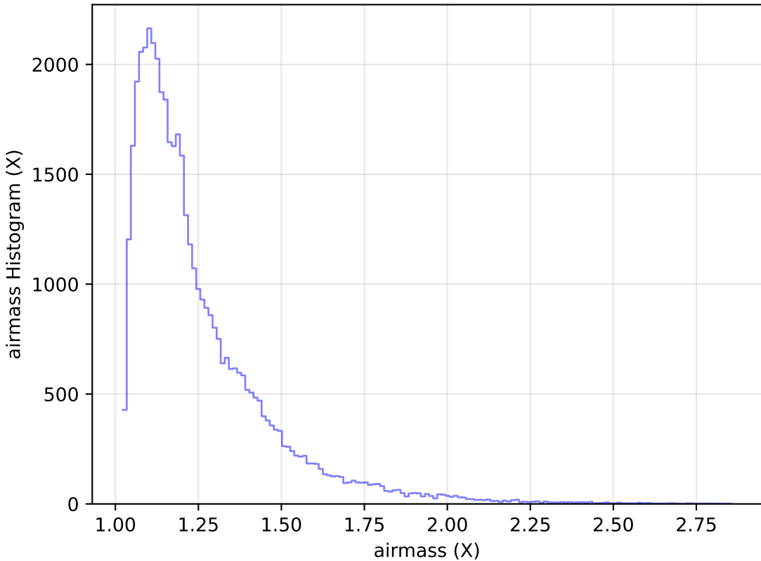
roll_pause_mjdp120_v3.4_10yrs Yr 1 y band: airmass Histogram
