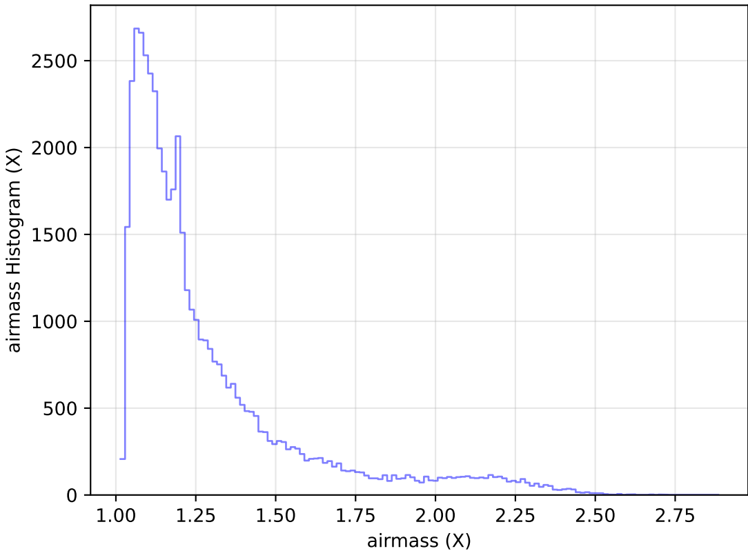
roll_pause_mjdp120_v3.4_10yrs Yr 1 r band: airmass Histogram
