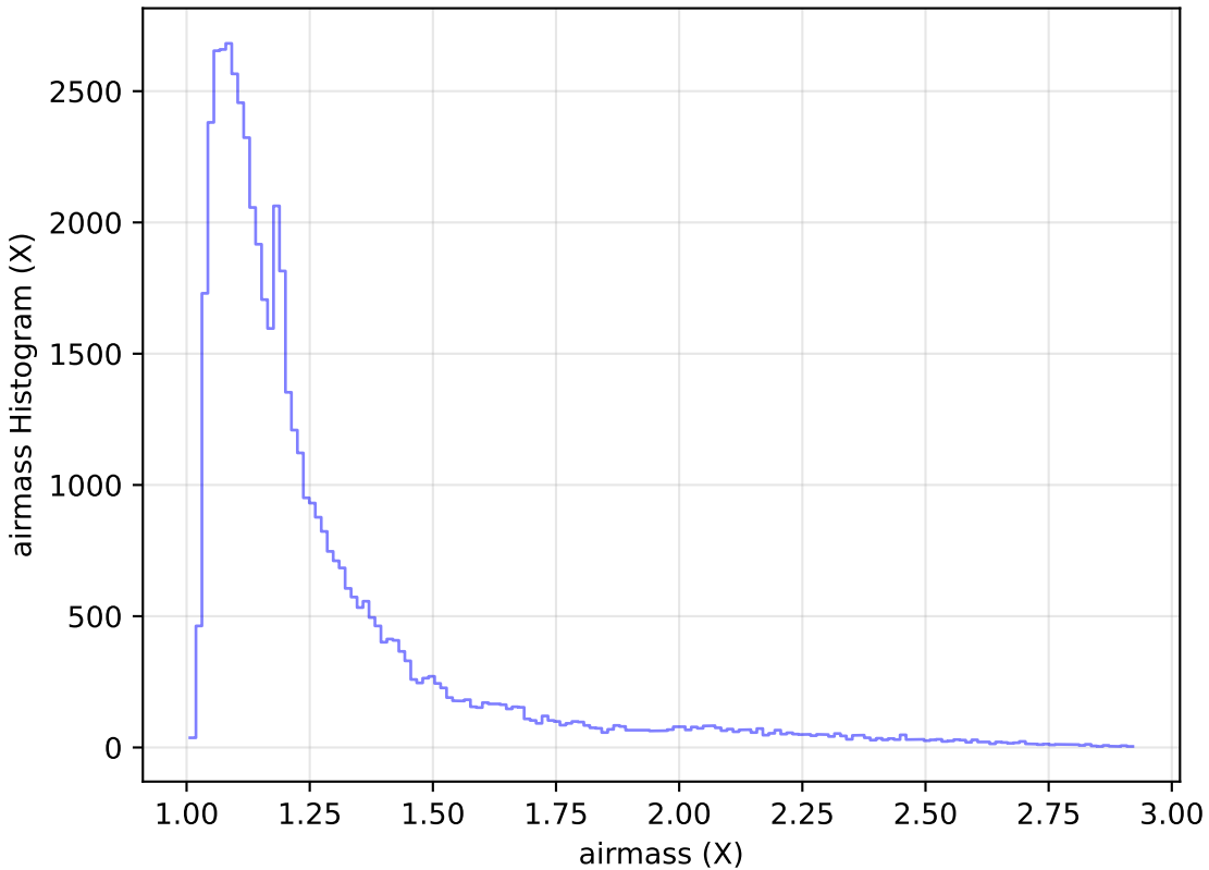
roll_pause_mjdp120_v3.4_10yrs Yr 1 i band: airmass Histogram
