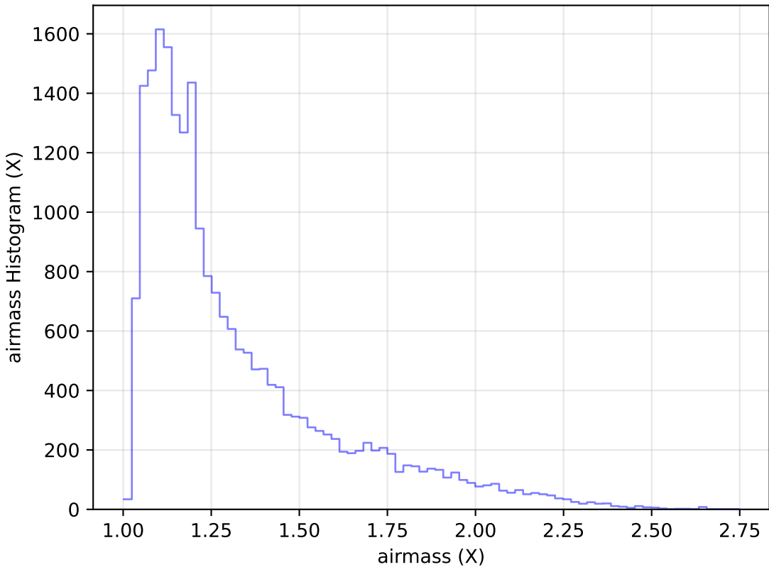
roll_pause_mjdp120_v3.4_10yrs Yr 1 g band: airmass Histogram
