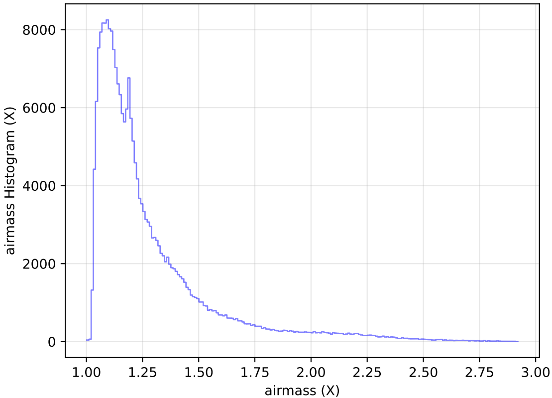
roll_pause_mjdp120_v3.4_10yrs Yr 1 all bands: airmass Histogram
