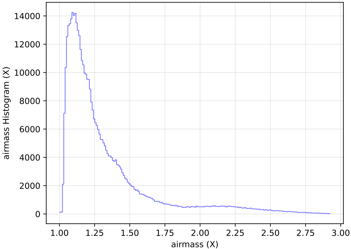
roll_pause_mjdp120_v3.4_10yrs WFD z band: airmass Histogram
