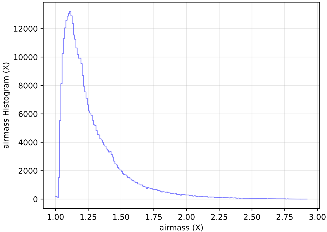
roll_pause_mjdp120_v3.4_10yrs WFD y band: airmass Histogram
