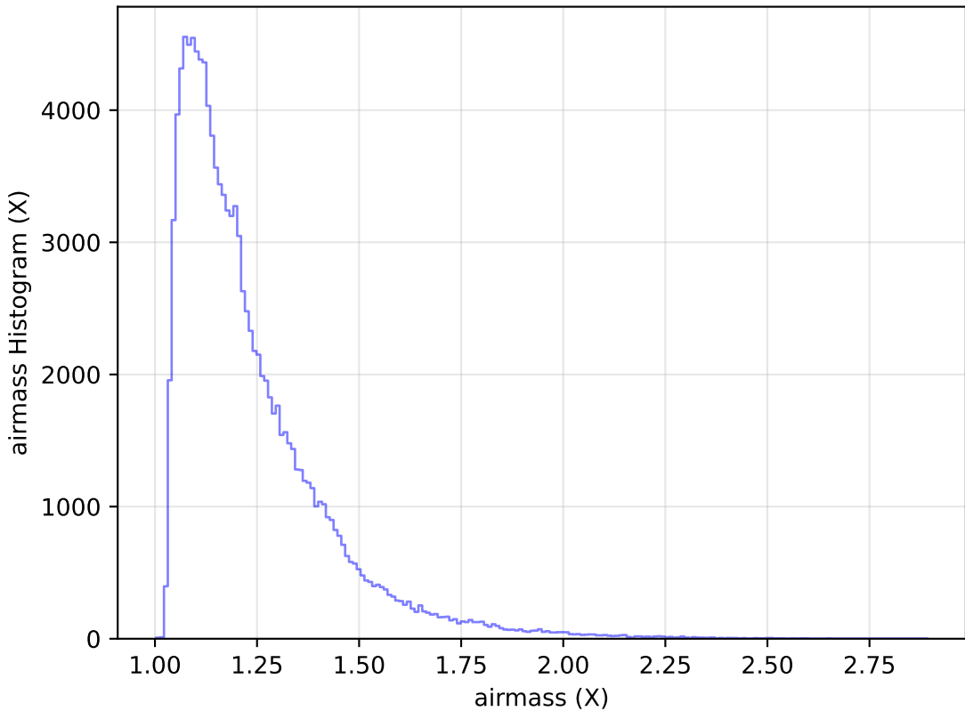
roll_pause_mjdp120_v3.4_10yrs WFD u band: airmass Histogram
