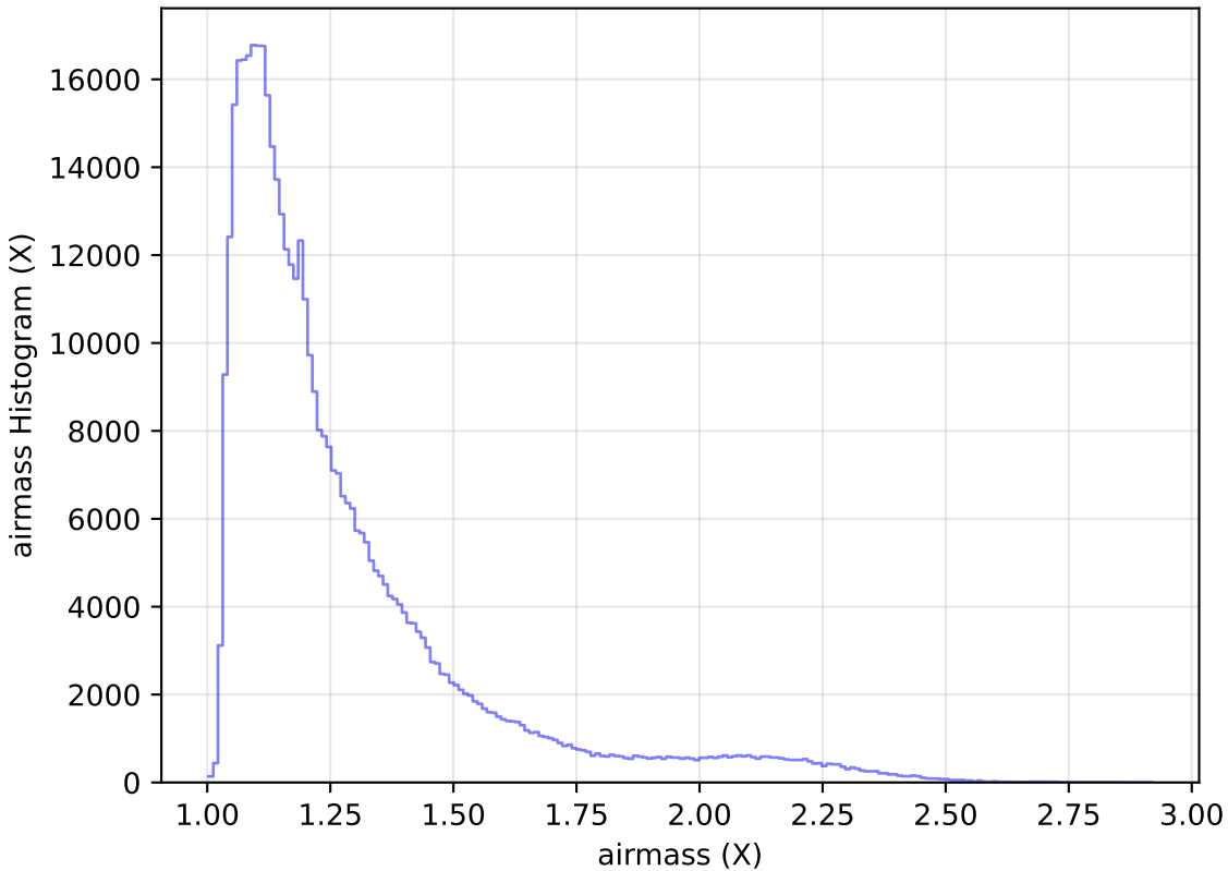
roll_pause_mjdp120_v3.4_10yrs WFD r band: airmass Histogram
