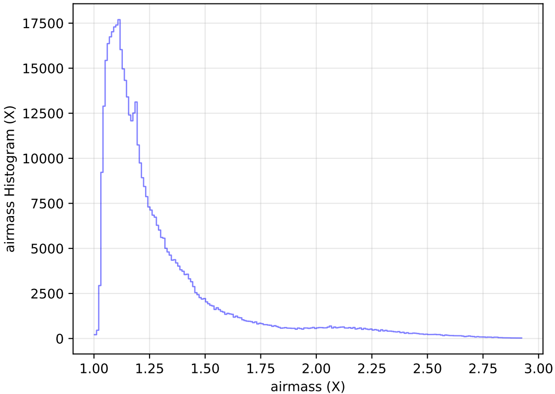
roll_pause_mjdp120_v3.4_10yrs WFD i band: airmass Histogram
