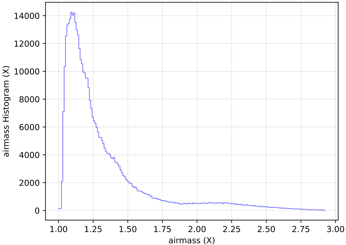
roll_pause_mjdp120_v3.4_10yrs All sky z band: airmass Histogram
