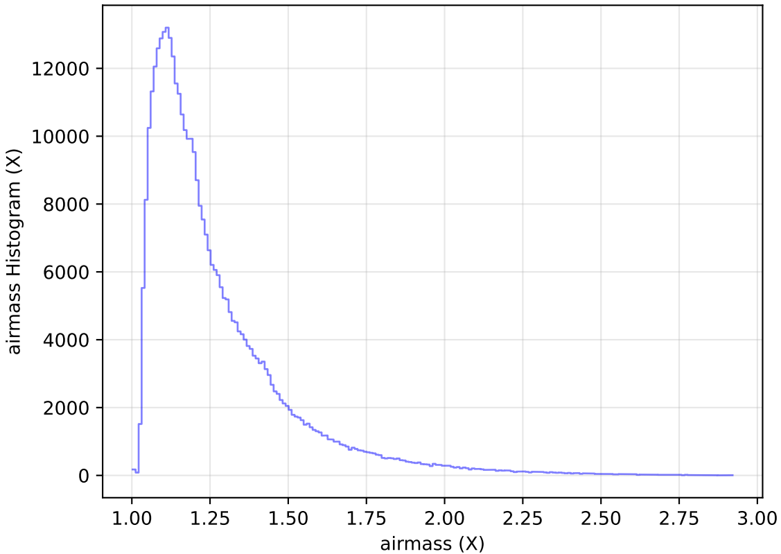
roll_pause_mjdp120_v3.4_10yrs All sky y band: airmass Histogram
