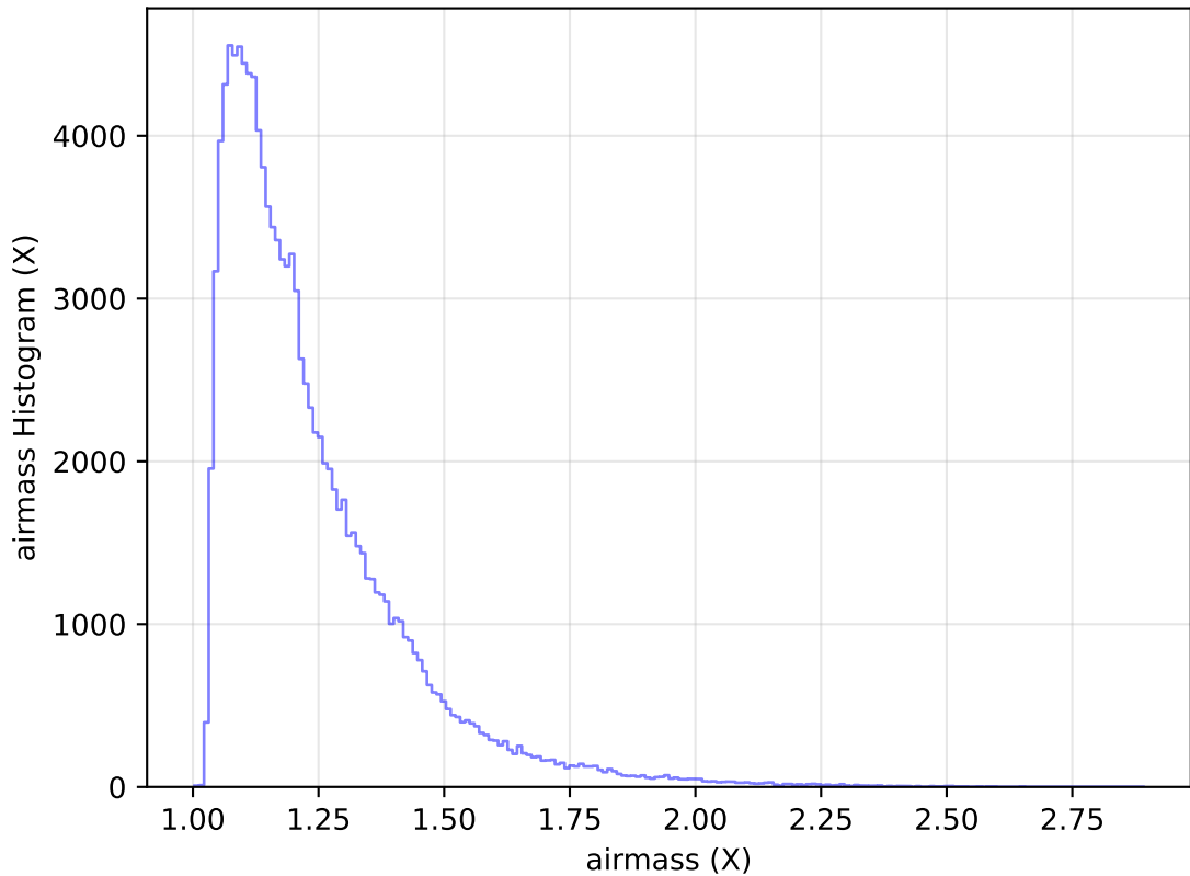
roll_pause_mjdp120_v3.4_10yrs All sky u band: airmass Histogram
