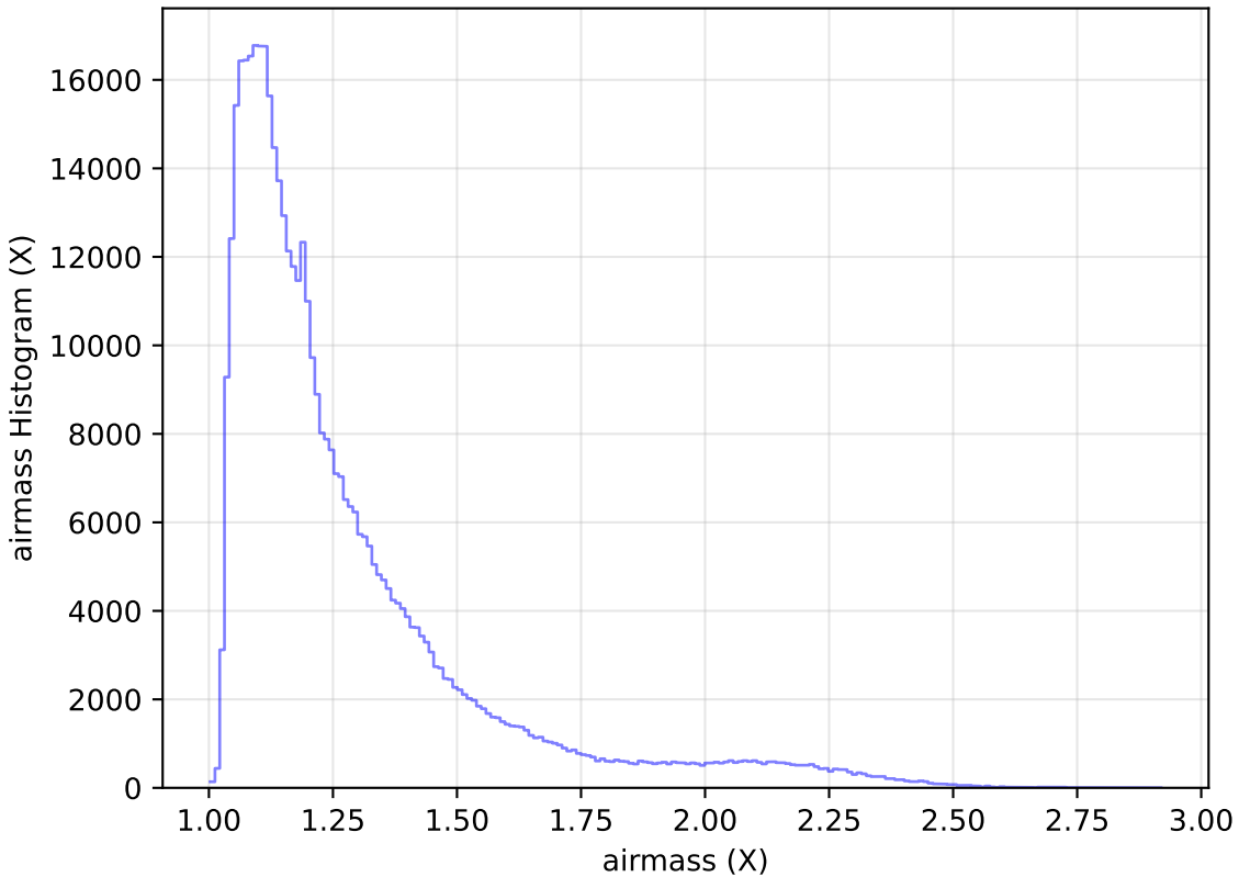
roll_pause_mjdp120_v3.4_10yrs All sky r band: airmass Histogram
