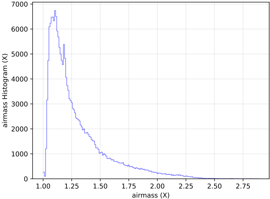
roll_pause_mjdp120_v3.4_10yrs All sky g band: airmass Histogram
