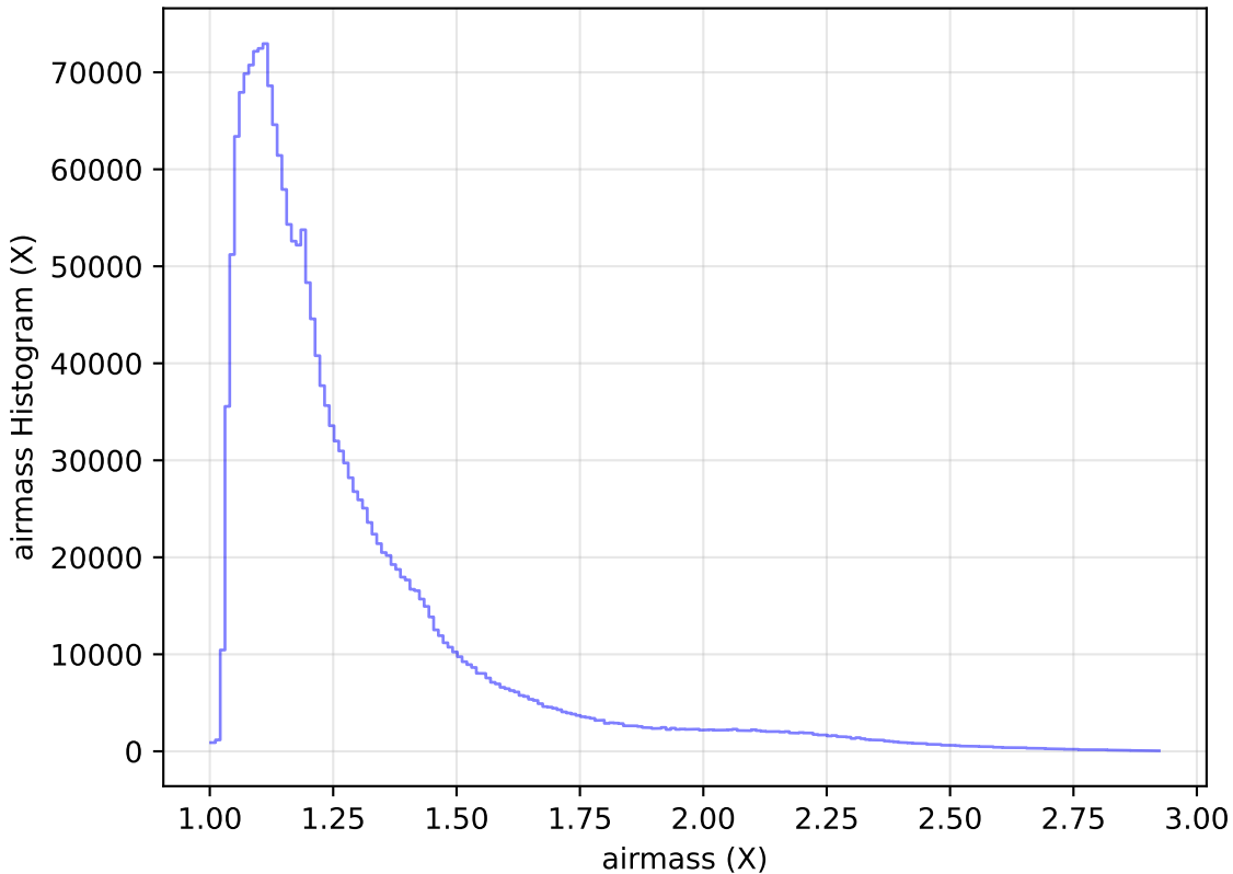
roll_pause_mjdp120_v3.4_10yrs All sky all bands: airmass Histogram
