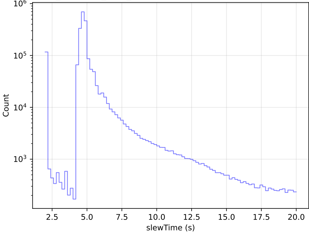
roll_pause_mjdp120_v3.4_10yrs All visits: Zoom Slew Time Histogram
