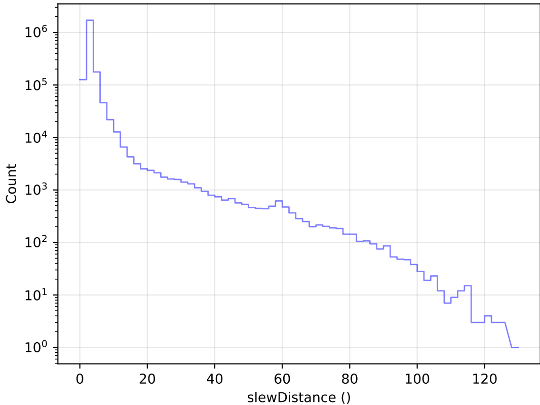
roll_pause_mjdp120_v3.4_10yrs All visits: Slew Distance Histogram
