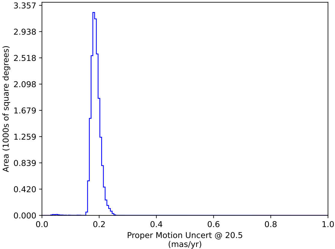
roll_pause_mjdp120_v3.4_10yrs WFD: Proper Motion Uncert @ 20.5
