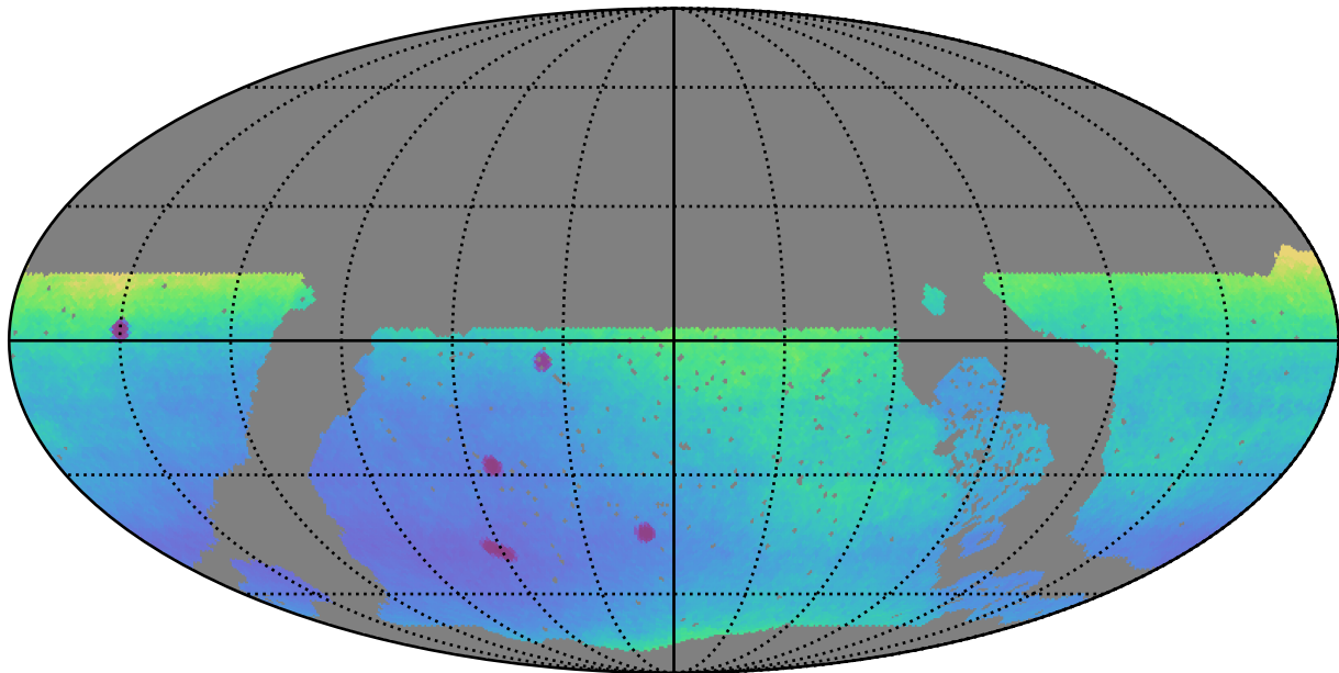
roll_pause_mjdp120_v3.4_10yrs WFD: Parallax Uncert @ 24.0
