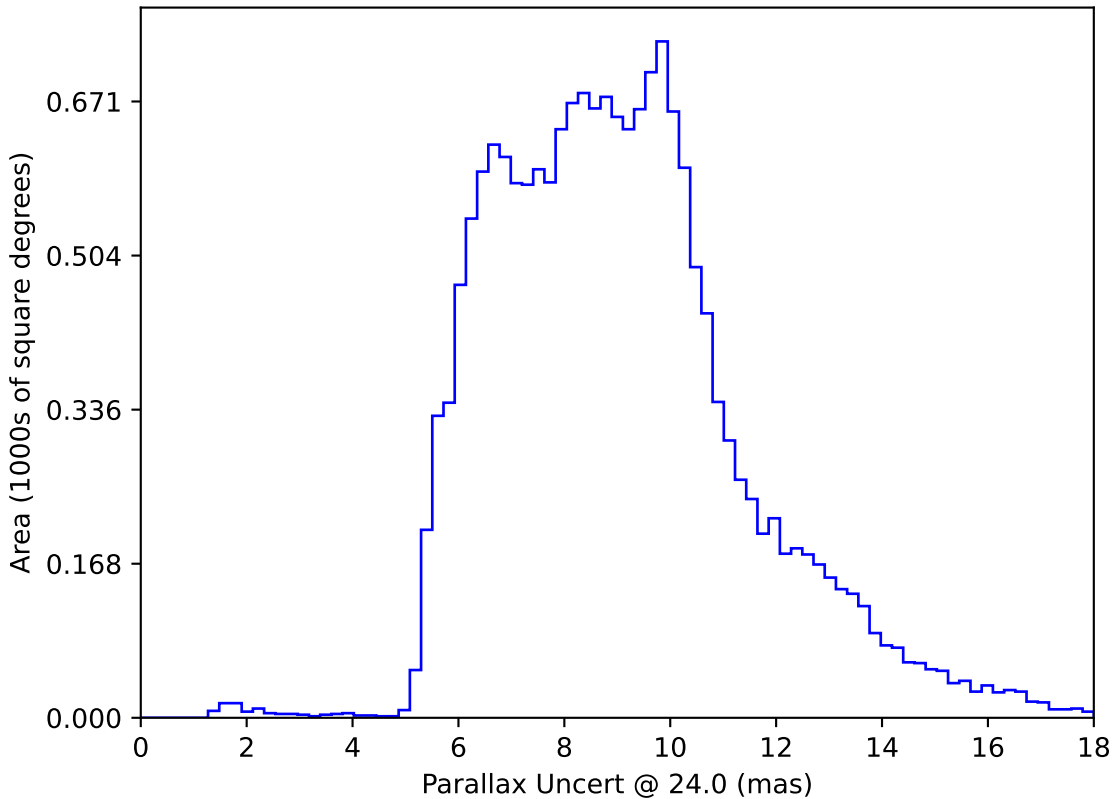
roll_pause_mjdp120_v3.4_10yrs WFD: Parallax Uncert @ 24.0
