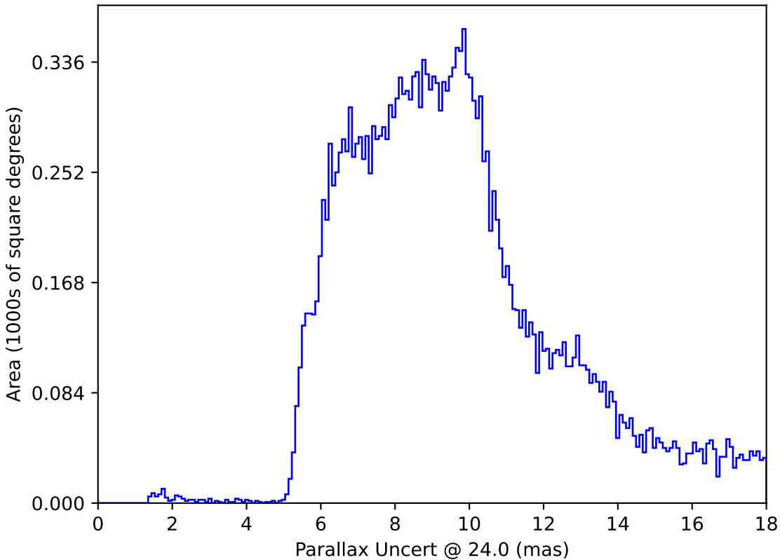
roll_pause_mjdp120_v3.4_10yrs All sky: Parallax Uncert @ 24.0
