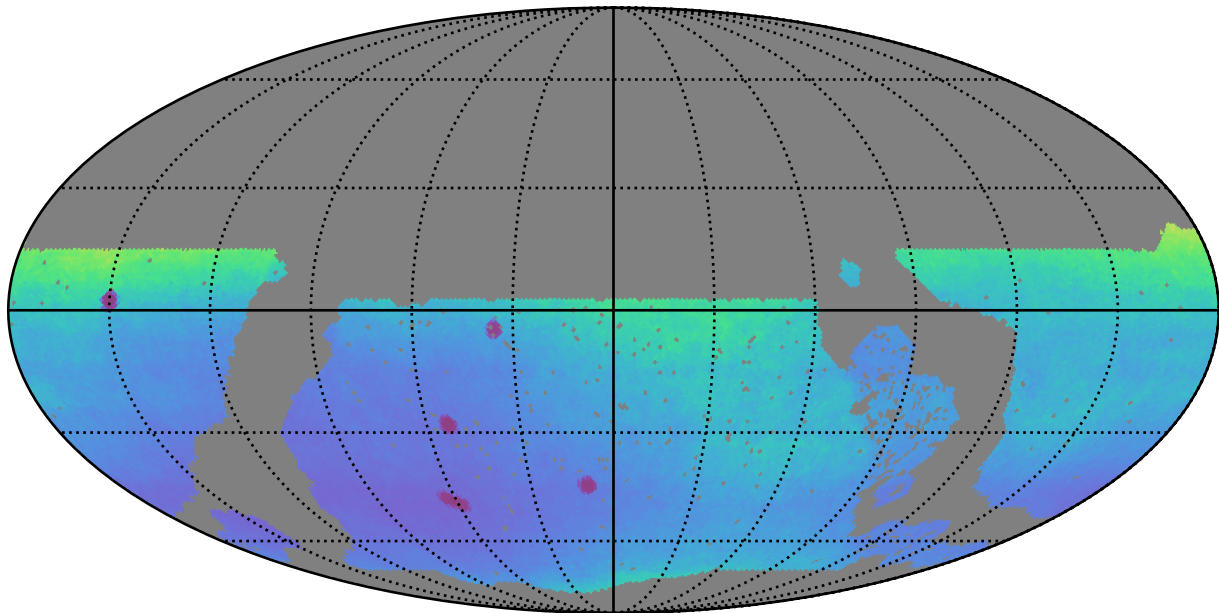
roll_pause_mjdp120_v3.4_10yrs WFD: Parallax Uncert @ 22.4
