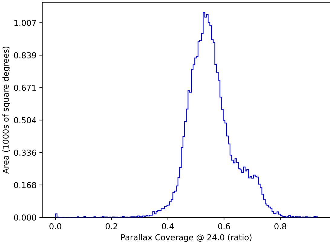
roll_pause_mjdp120_v3.4_10yrs All sky: Parallax Coverage @ 24.0
